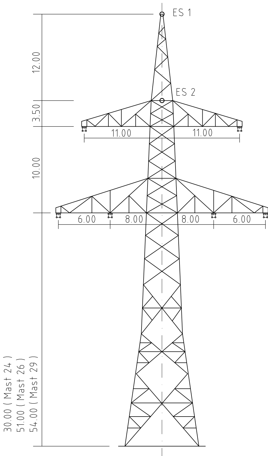
Mast Nr. 24, 26, 29
