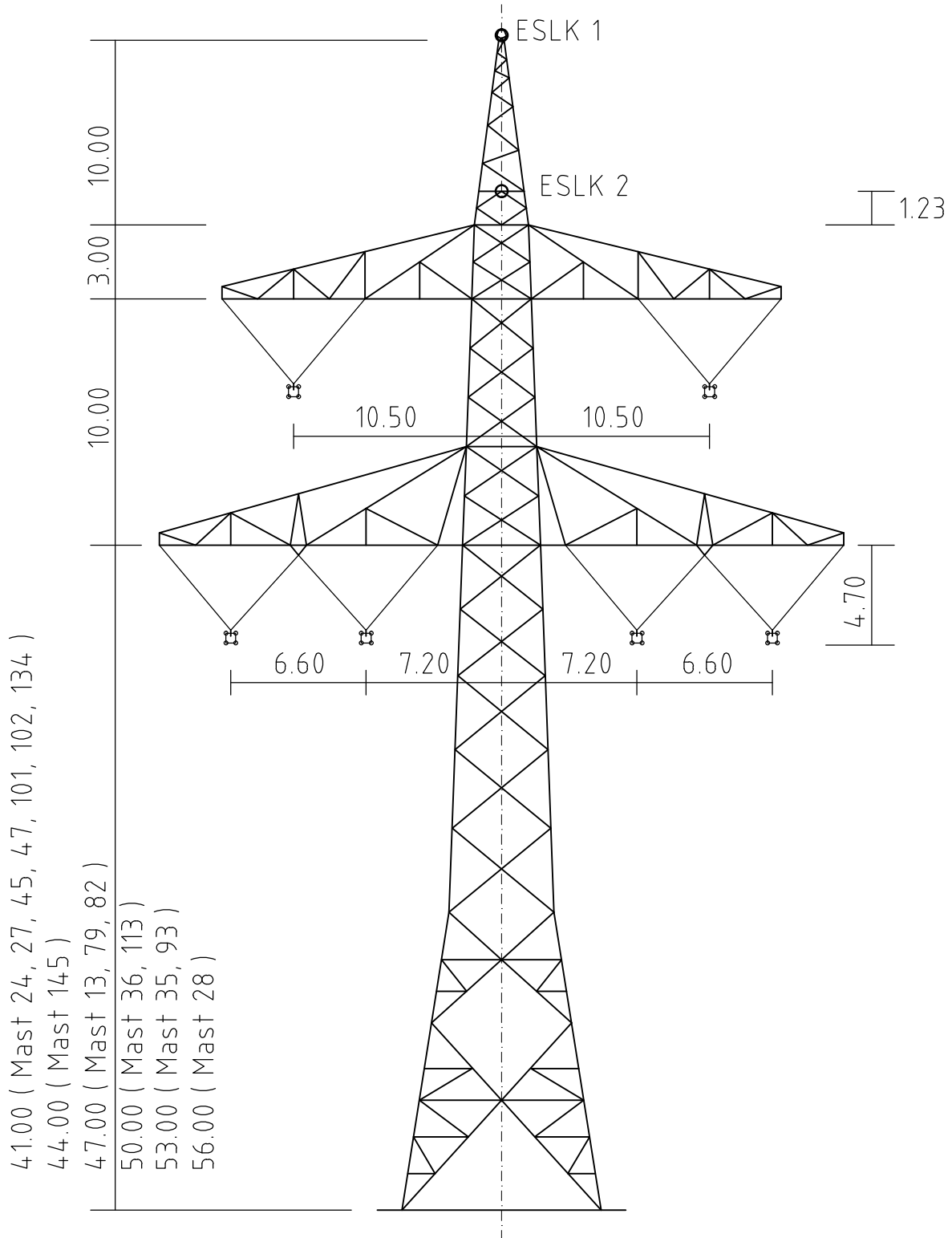
Mast Nr. 13, 24, 27, 28, 35, 36, 45, 47, 79, 82, 93, 101, 102, 113, 134, 145
